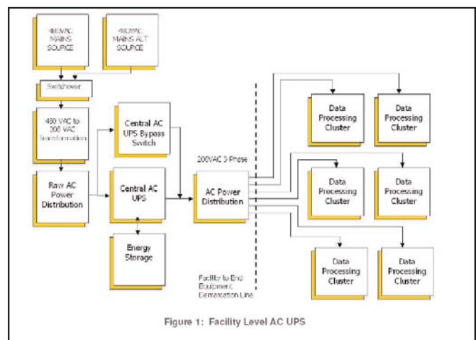
Figure 1: Facility Level AC UPS
